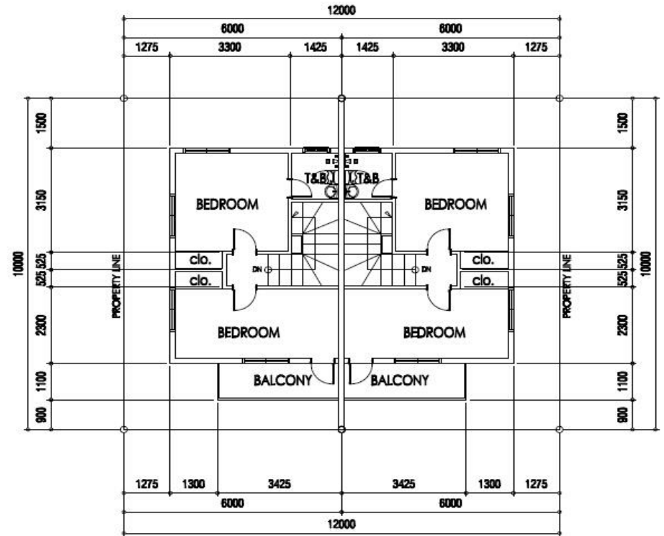
2 SECOND FLOOR PLAN A-2 SCALE: 1:100 MTS
