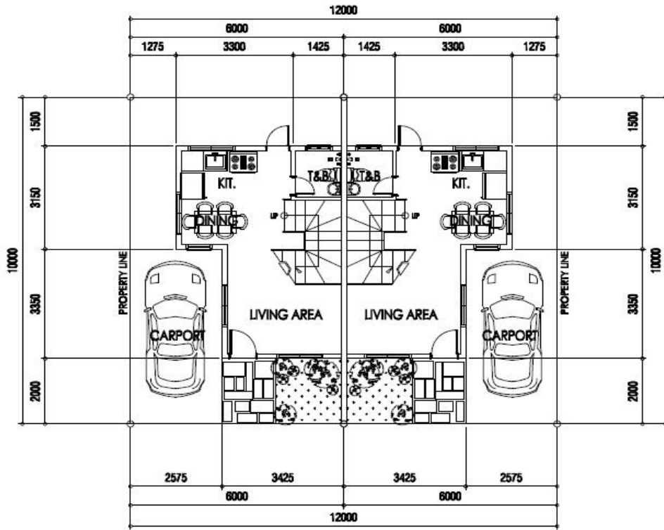
1 GROUND FLOOR PLAN A-2 SCALE: 1:100 MTS
